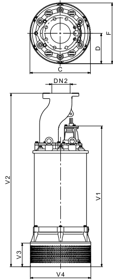
Flange connection
