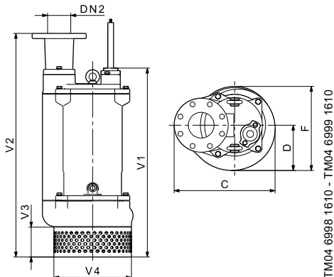
Flange connection
