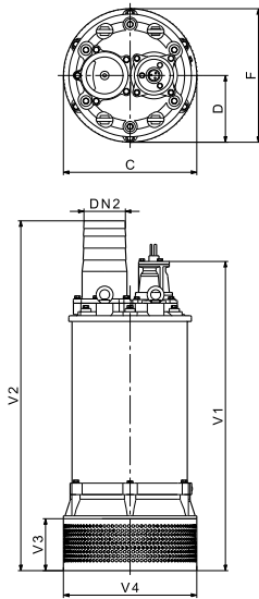
Hose connection
